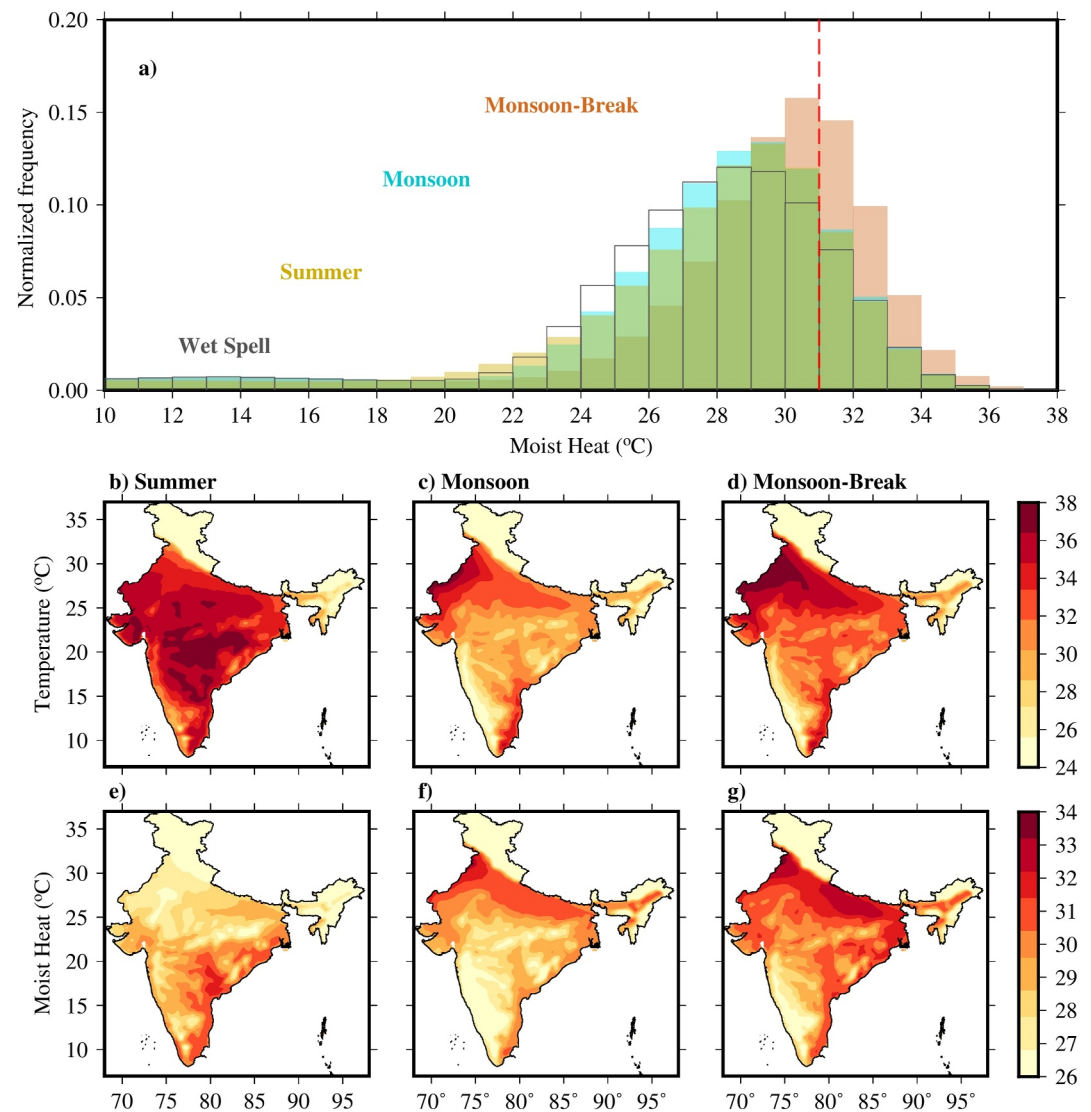
Figure 1. Observed extreme moist heat (Wet-Bulb Globe Temperature (WBGT)) during Monsoon-Break. (a) Normalized frequency for summer, monsoon and monsoon-break annual mean (6 hr mean daily maximum) during the 1951–2020 period, (b) summer season (March, April, and May) 6 hr mean daily maximum temperature for the same period as (a), (c) same as panel (b) but for monsoon season (June, July, August, and September), (d) same as panel (b) but for monsoon break, and (e–g) same as panels (b–d) but for moist heat. The moist heat is derived from daily maximum of 6 hr mean WBGT. Here, monsoon season does not include break period.
