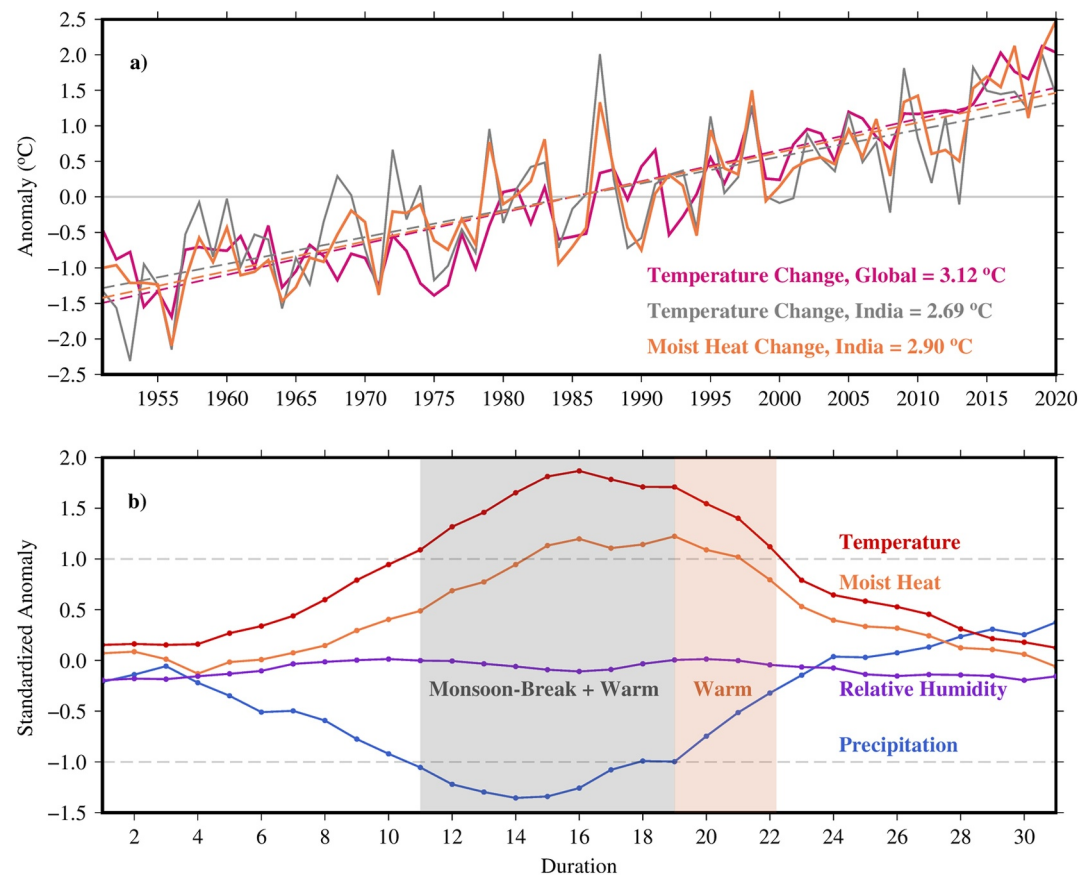
Figure 3. Drivers of moist heat (Wet-Bulb Globe Temperature) extremes in India. (a) Mean temperature and moist heat anomalies and their trends for the globe and India during the 1951–2020 monsoon (JJAS) period and (b) mean anomaly composite during the break period for the 1951–2020 period. (b) is calculated for the 30-day buffer period. The buffer period is calculated from the middle of a break period, including 15 previous and ahead days. Here, only a break period (including warm and monsoon break) of 7 days or longer is considered for the calculation.
