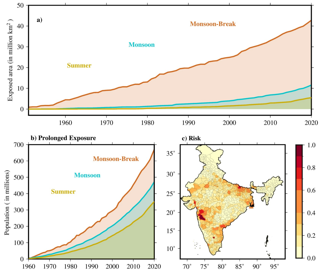
Figure 2. Moist heat (Wet-Bulb Globe Temperature) exceedance and risk for India. (a) Accumulated surface area experiencing 31°C moist heat exceedance for at least six continuous hours for the 1951–2020 period, (b) population exposed to 31°C moist heat exceedance for at least six continuous hours during the 1960–2020 period, and (c) district (official boundary) wise extreme moist heat risk for the 1951–2020 period. The risk is calculated from the product of vulnerability, population, and hazard (described in text). The area exposed to exceedance is calculated for each year.
